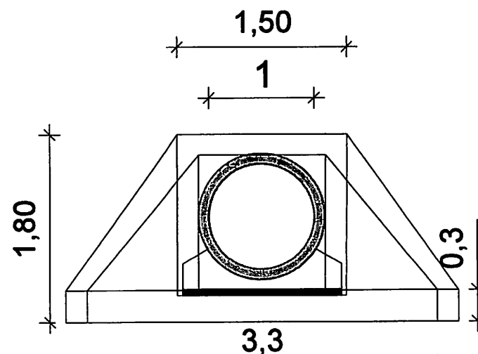
VISTA FRONTAL BOCA BSTC - 1,00M
